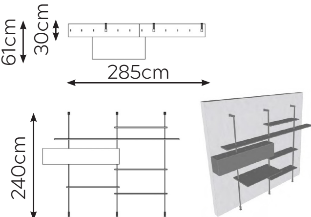
WALL WITH DESK (COMPOSITION 3-010) W: 285cm D: 61cm H: 240cm
