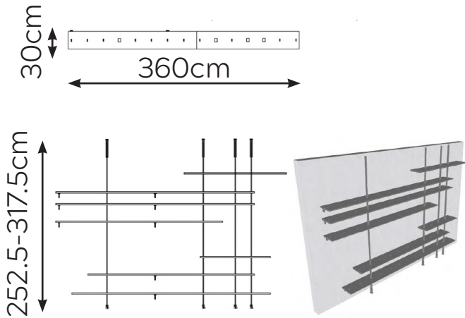
CEILING (COMPOSITION 4-001) W: 360cm D: 30cm H: 252.5-317.5cm
