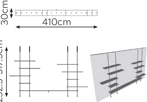
CEILING (COMPOSITION 4-003) W: 410cm D: 30cm H: 252.5-317.5cm
